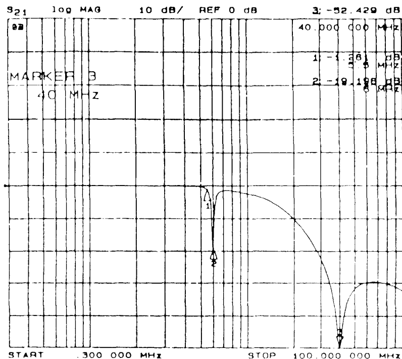
Fig.3 Video Filter response.
